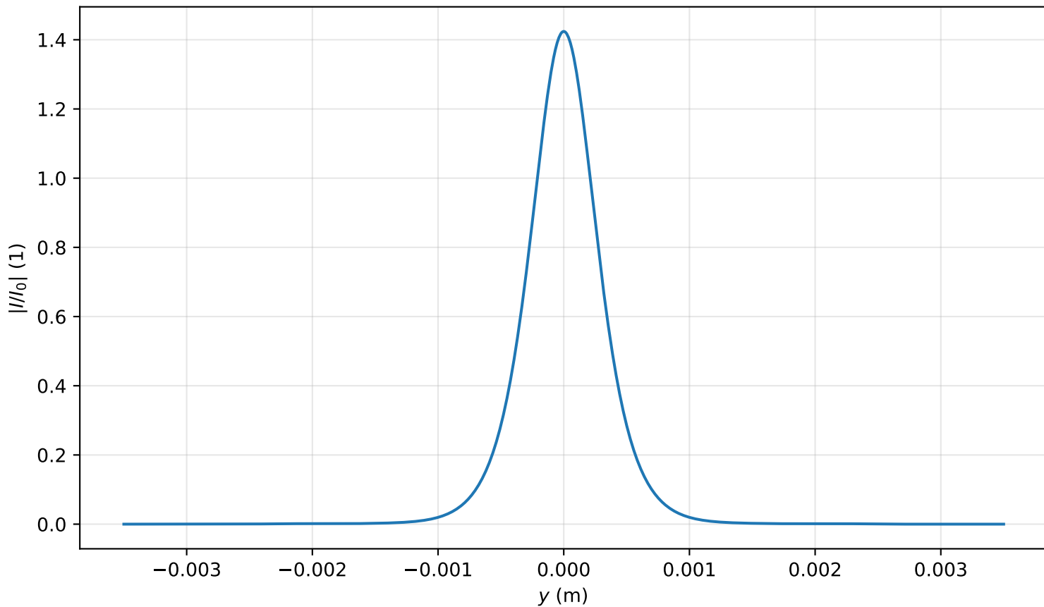
Intensity profile I(x=0, y, z=3.901)/I_0 , P_{in}=0.9P_{cr} , artificial time
